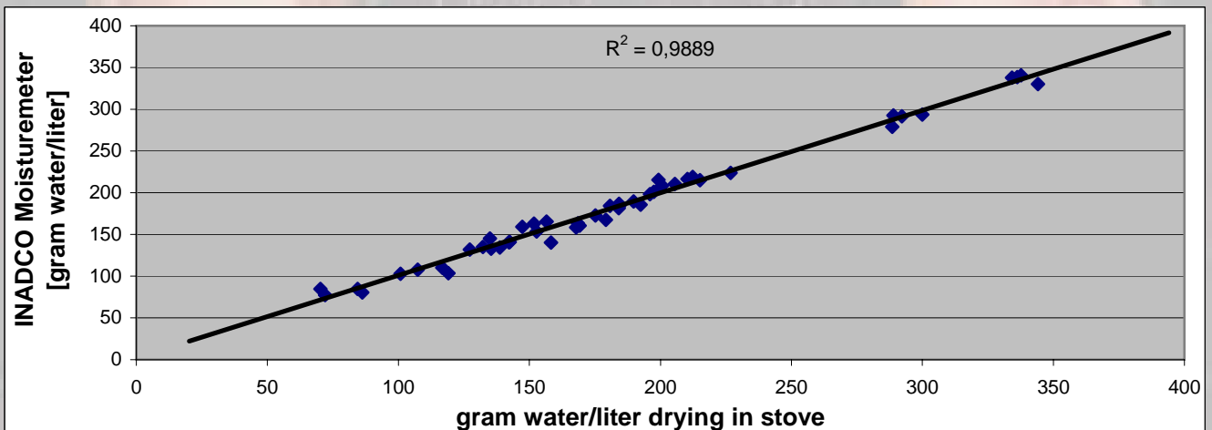
Results of the INADCO Moisturemeter compared with the method of drying in a stove
